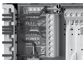
Conductivity probe ① yellow ② transparent
