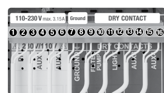
Setup and connection of a Variable Speed Pump, see section 13 - Variable Speed Pump
